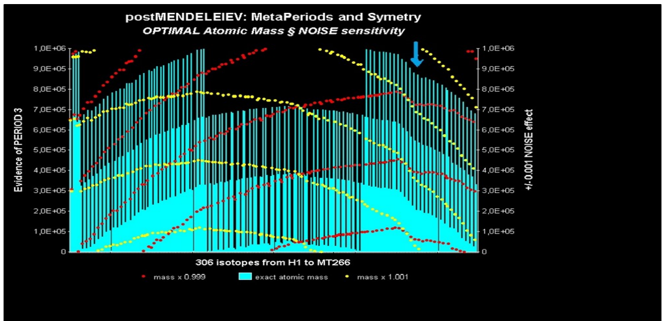
Figure 32. Symmetry of the PI-masses of the 306 successive isotopes of the Mendeleev Elements table.
